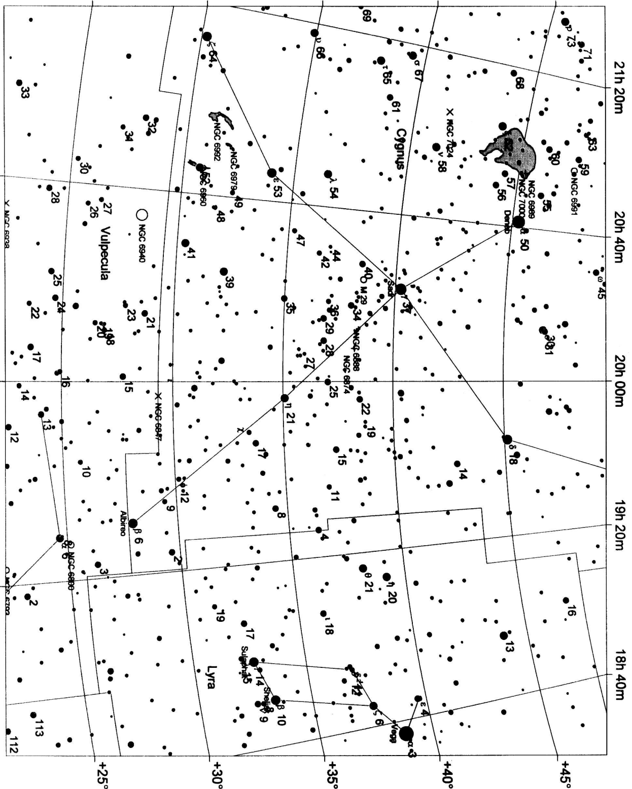
Cygnus -- 'Albireo' Beta (6) Cygni, North American Nebula (NGC 7000) etc. etc
