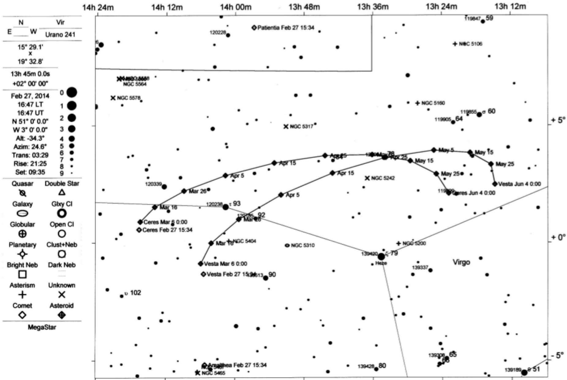
1 Ceres & 4 Vesta in Virgo. March 6 to June 4 2014. 10 day intervals.
