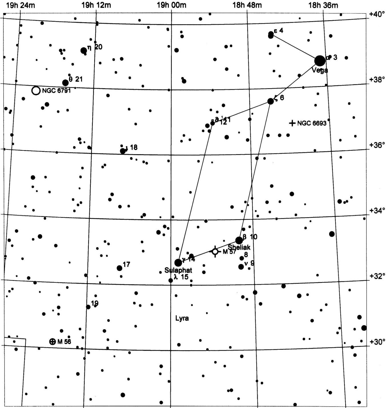
M57 (NGC 6720) etc. in Lyra.
